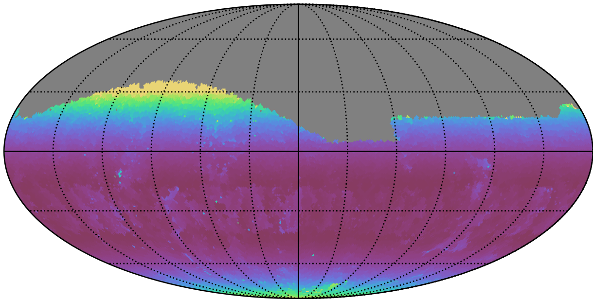
weather_cloudso14v3.4_10yrs Yr 1 g band: Min airmass
