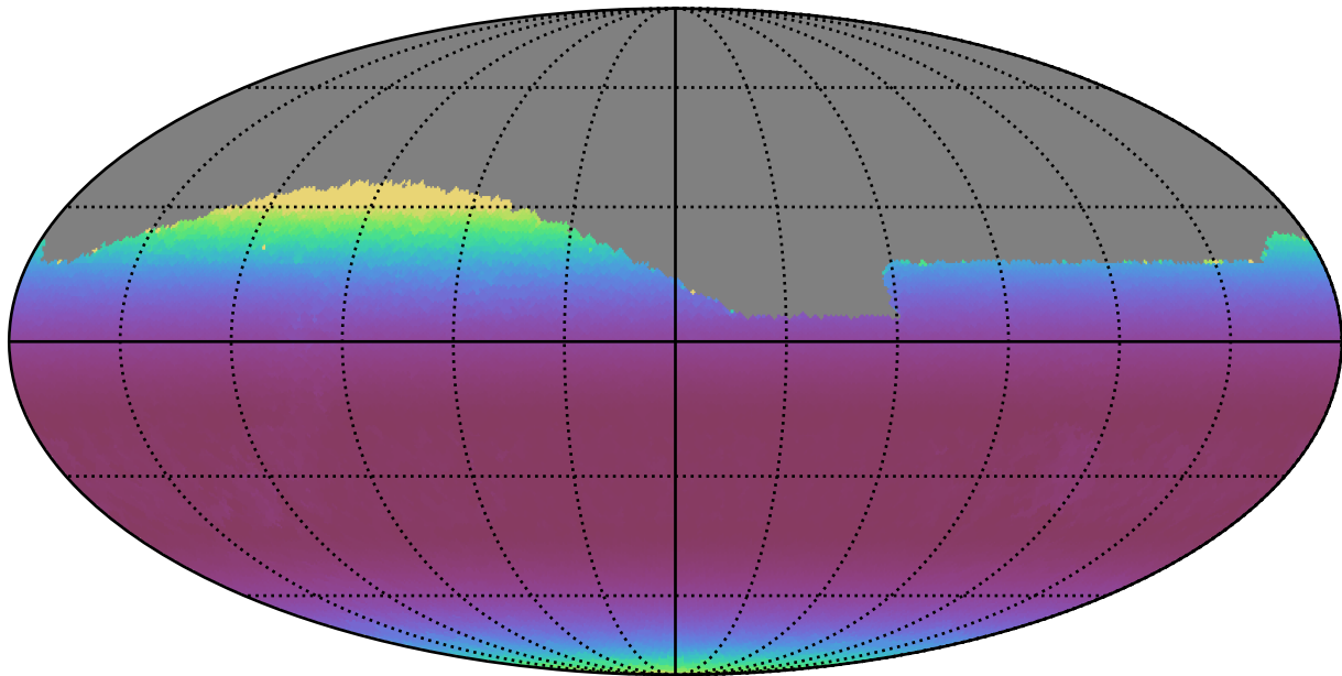
weather_cloudso14v3.4_10yrs Yr 1 all bands: Min airmass
