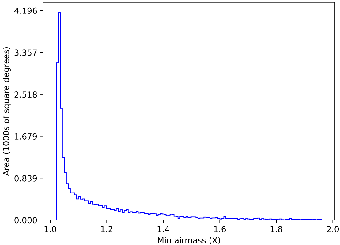
weather_cloudso14v3.4_10yrs Yr 1 all bands: Min airmass
