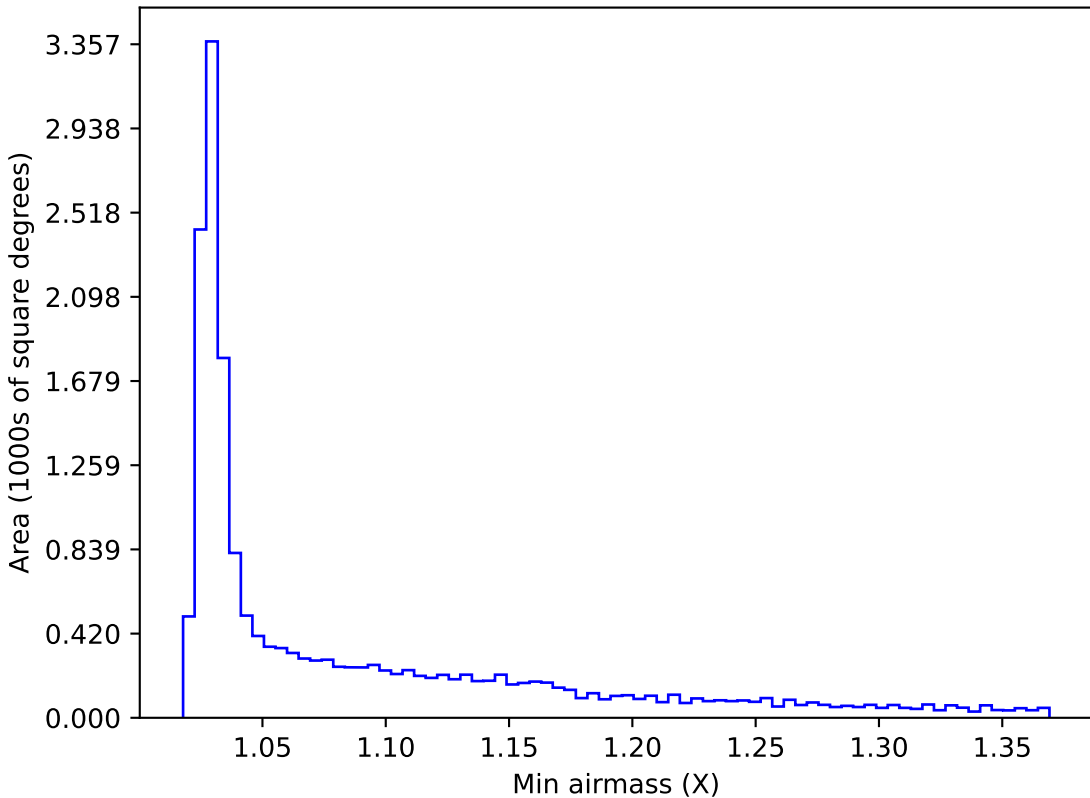
weather_cloudso14v3.4_10yrs WFD z band: Min airmass
