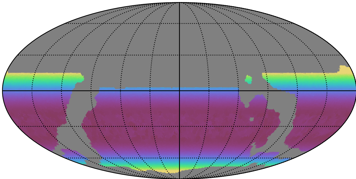
weather_cloudso14v3.4_10yrs WFD r band: Min airmass
