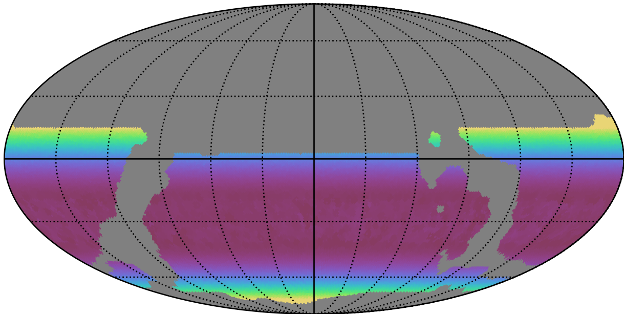
weather_cloudso14v3.4_10yrs WFD i band: Min airmass
