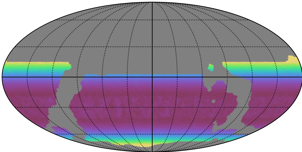
weather_cloudso14v3.4_10yrs WFD g band: Min airmass
