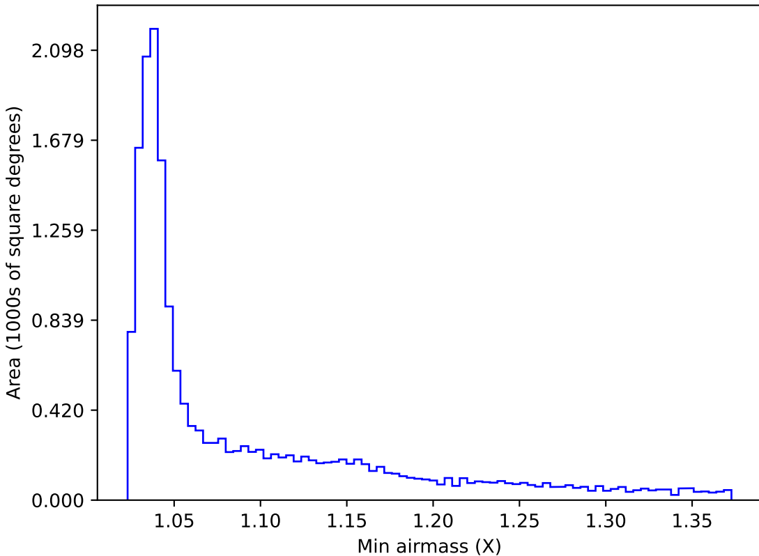
weather_cloudso14v3.4_10yrs WFD g band: Min airmass
