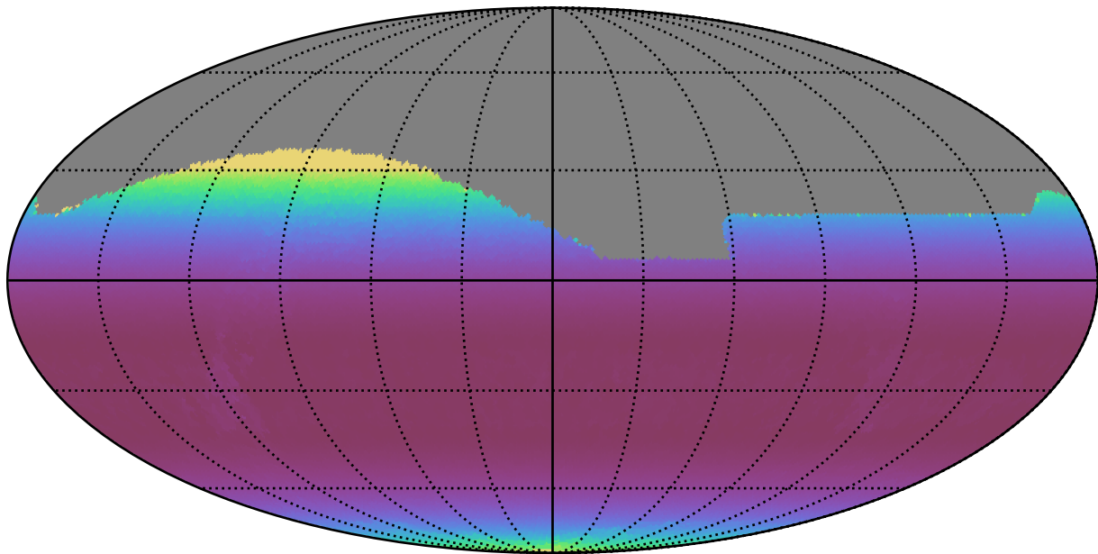
weather_cloudso14v3.4_10yrs All sky z band: Min airmass
