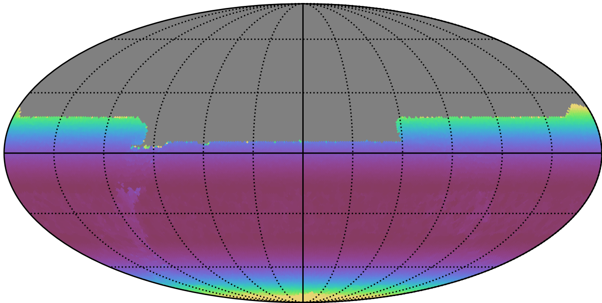
weather_cloudso14v3.4_10yrs All sky y band: Min airmass
