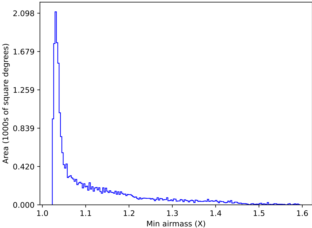
weather_cloudso14v3.4_10yrs All sky y band: Min airmass
