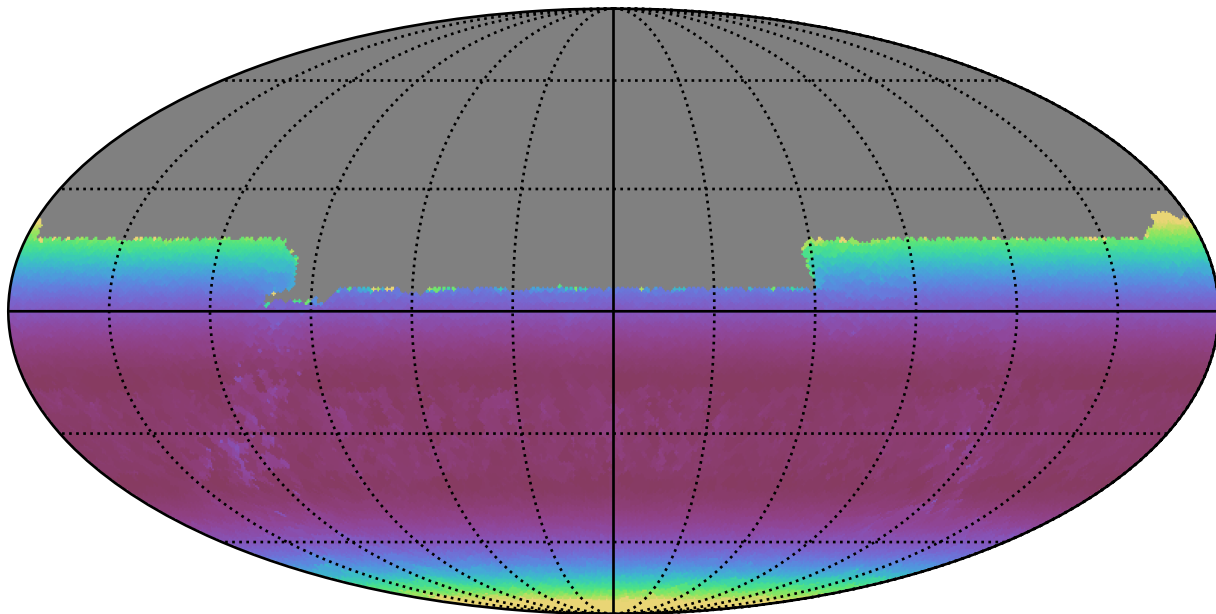
weather_cloudso14v3.4_10yrs All sky u band: Min airmass
