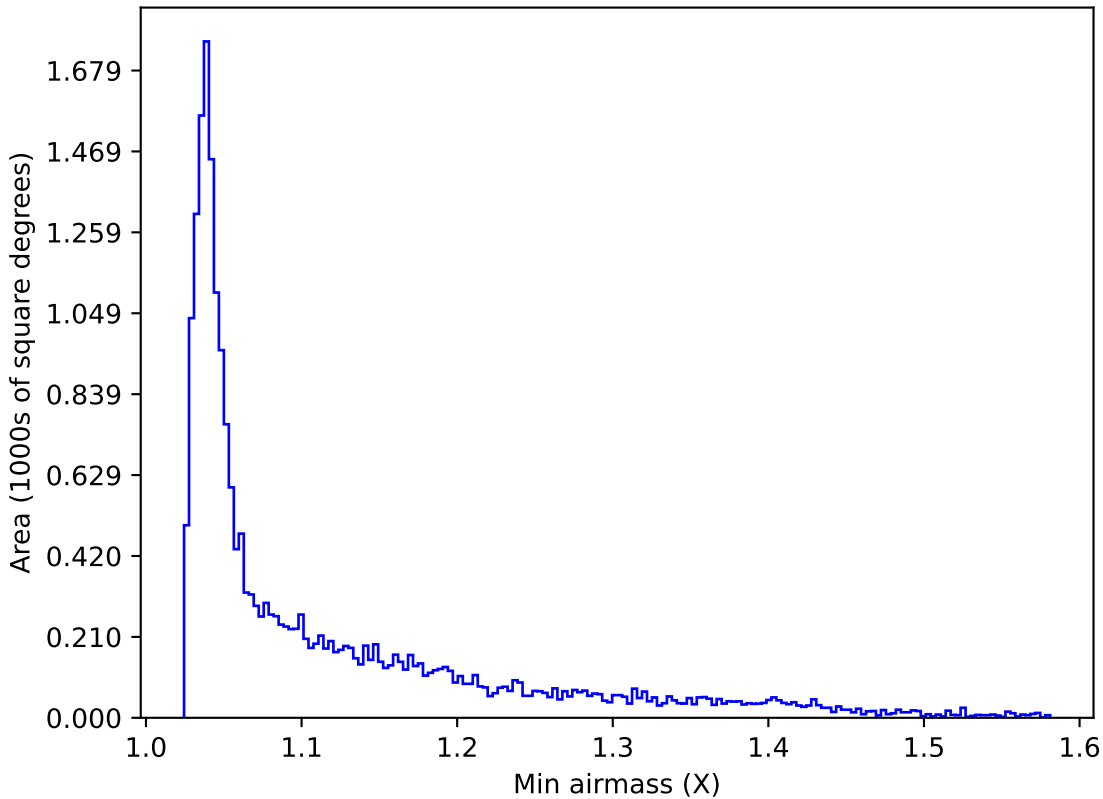
weather_cloudso14v3.4_10yrs All sky u band: Min airmass
