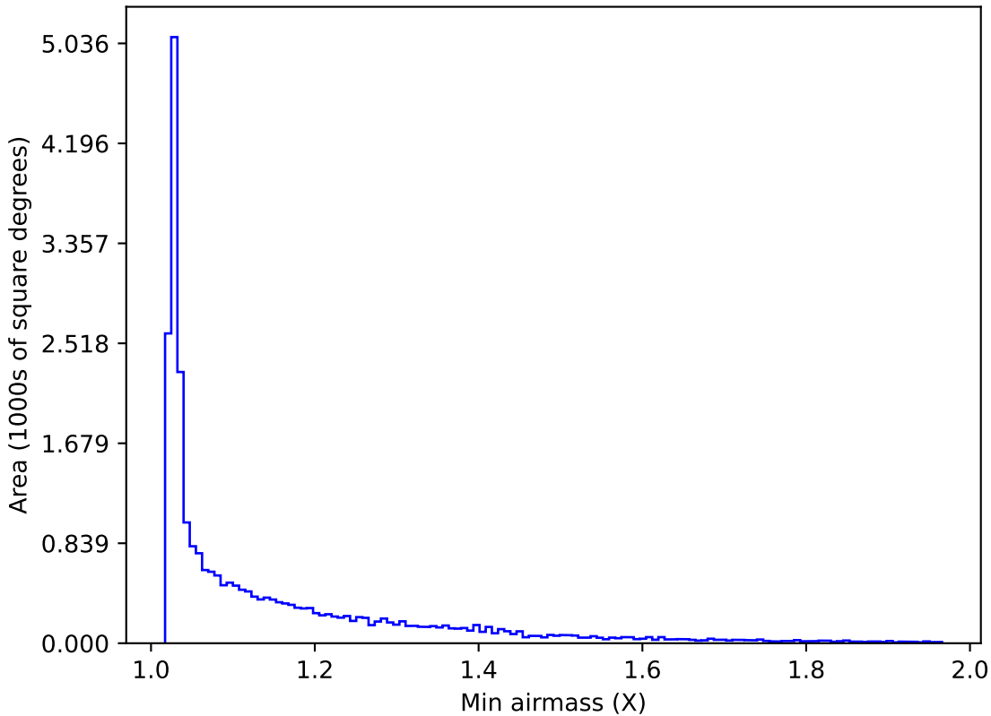
weather_cloudso14v3.4_10yrs All sky r band: Min airmass
