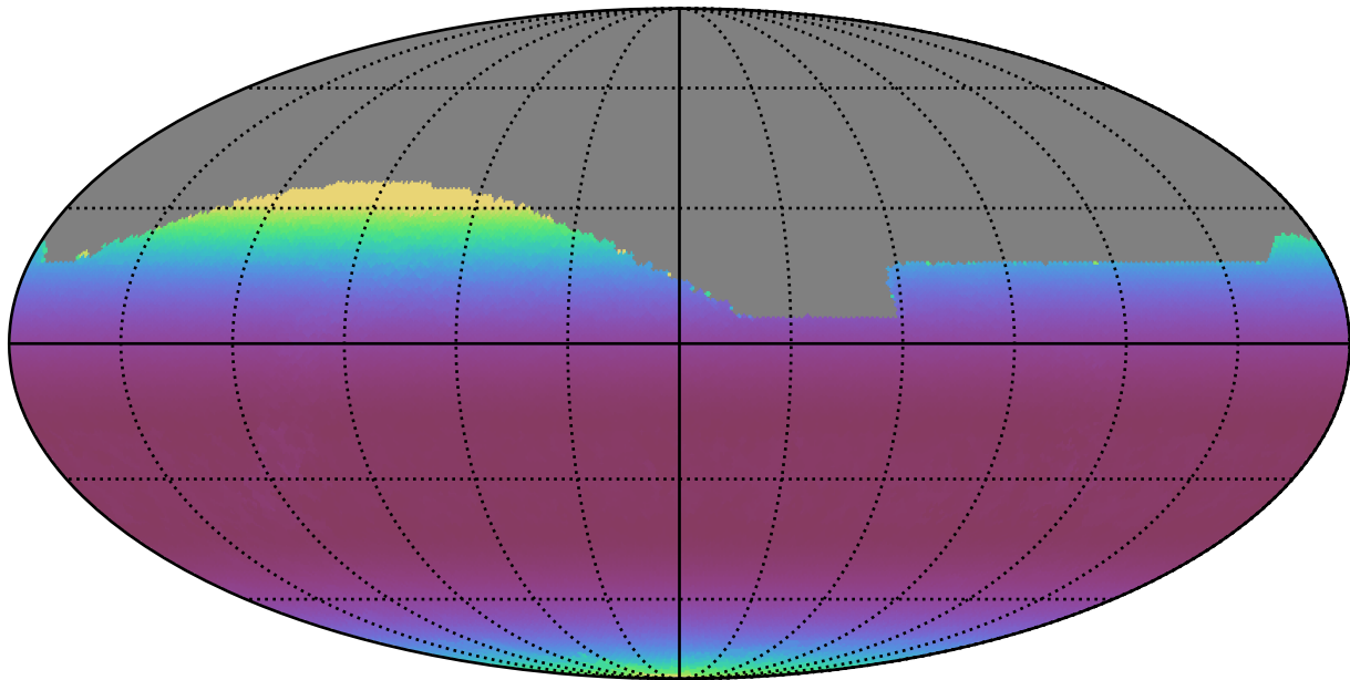
weather_cloudso14v3.4_10yrs All sky i band: Min airmass
