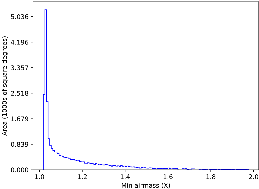
weather_cloudso14v3.4_10yrs All sky i band: Min airmass
