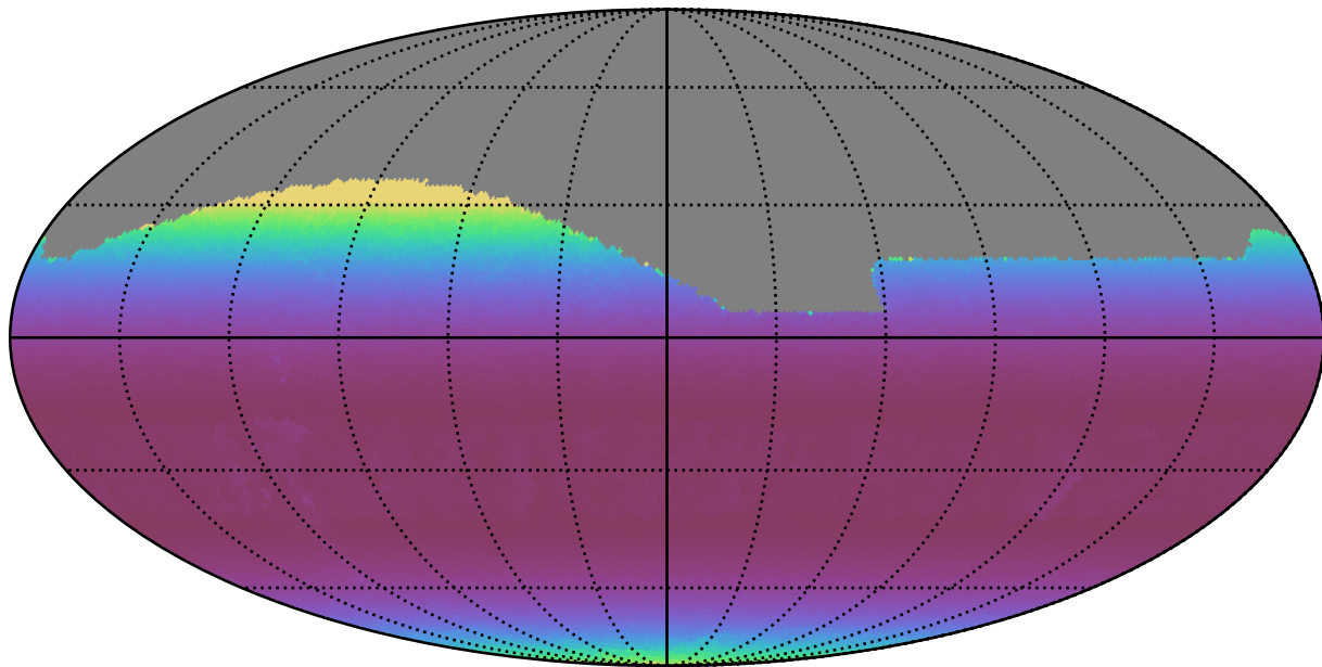
weather_cloudso14v3.4_10yrs All sky g band: Min airmass
