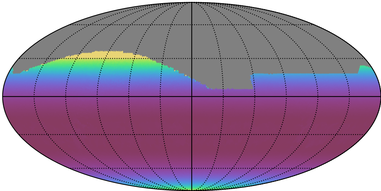
weather_cloudso14v3.4_10yrs All sky all bands: Min airmass
