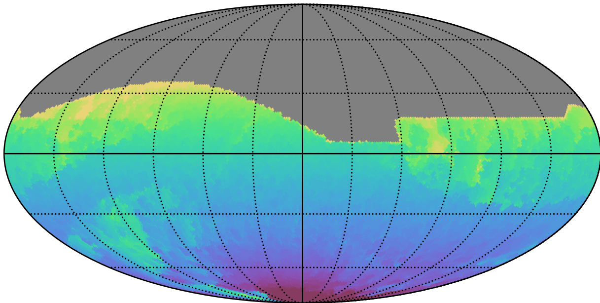
weather_cloudso14v3.4_10yrs All sky all bands: Min HA
