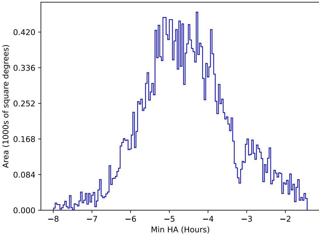
weather_cloudso14v3.4_10yrs All sky all bands: Min HA
