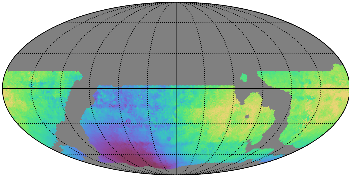
weather_cloudso14v3.4_10yrs WFD z band: Median solarElong
