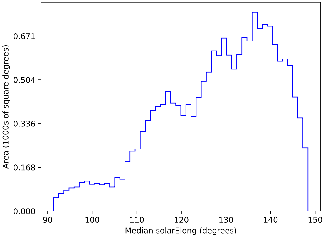
weather_cloudso14v3.4_10yrs WFD z band: Median solarElong
