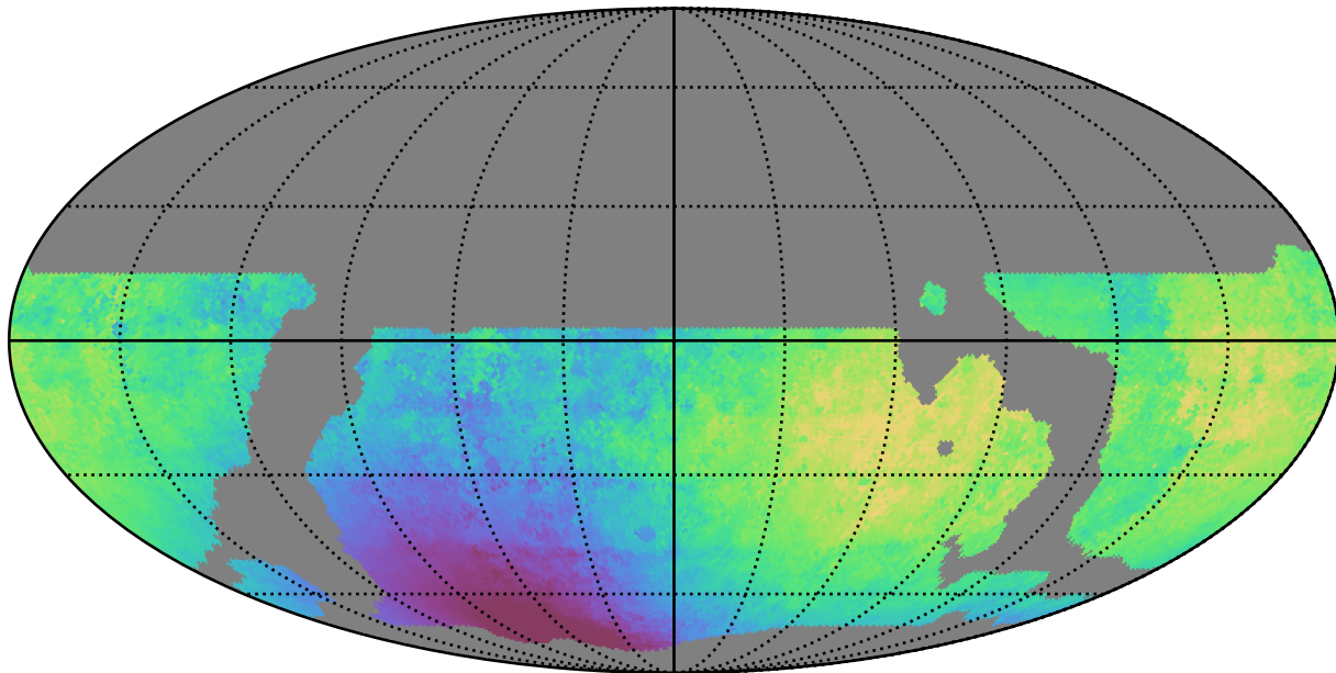
weather_cloudso14v3.4_10yrs WFD y band: Median solarElong
