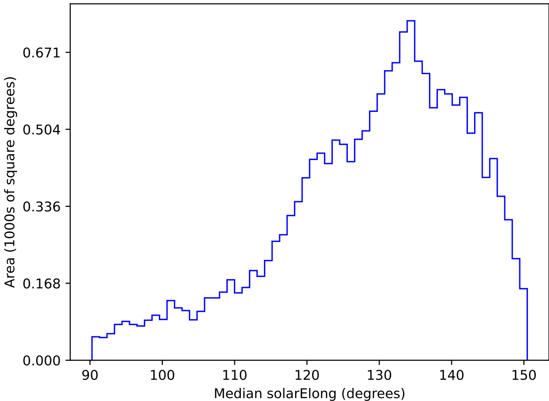
weather_cloudso14v3.4_10yrs WFD y band: Median solarElong
