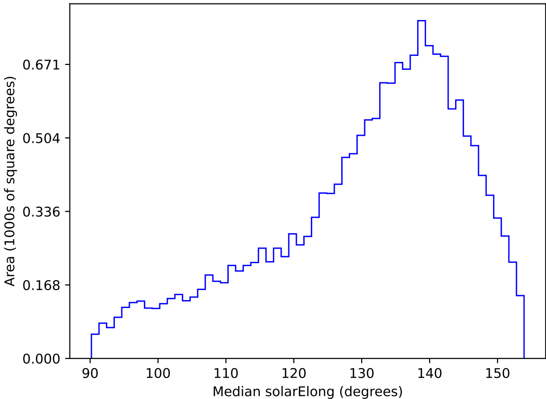
weather_cloudso14v3.4_10yrs WFD u band: Median solarElong
