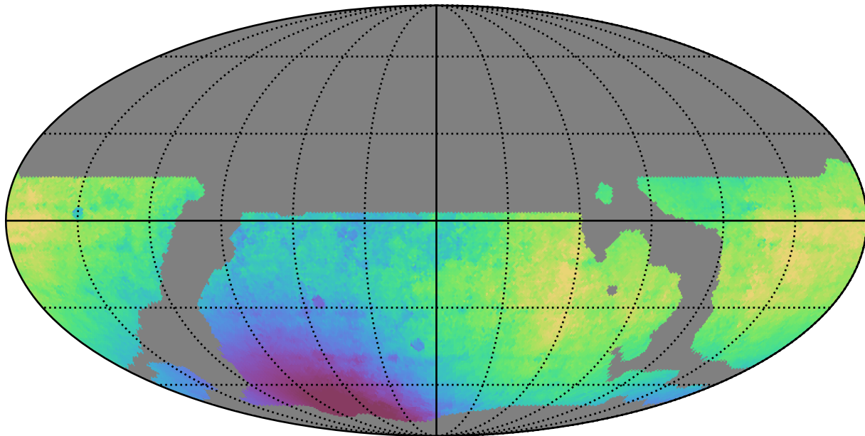
weather_cloudso14v3.4_10yrs WFD r band: Median solarElong
