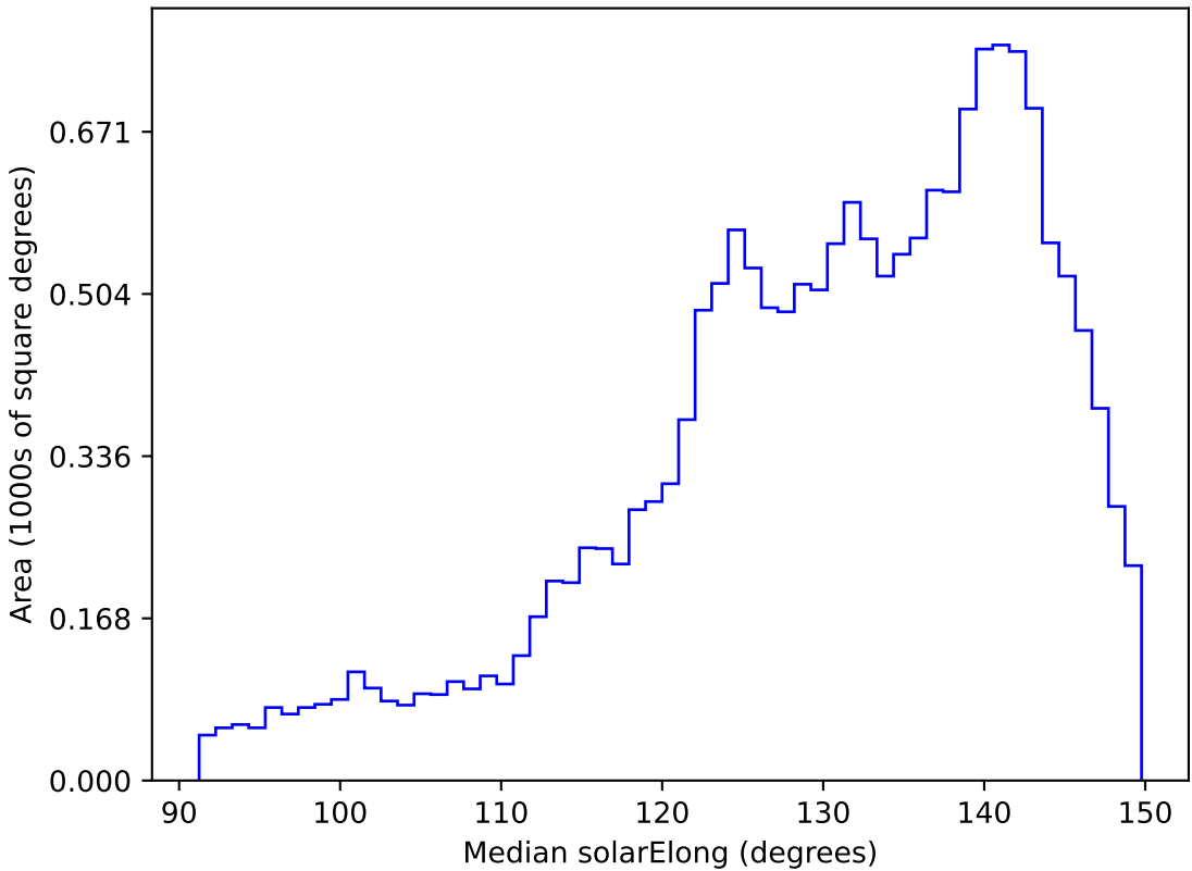
weather_cloudso14v3.4_10yrs WFD r band: Median solarElong
