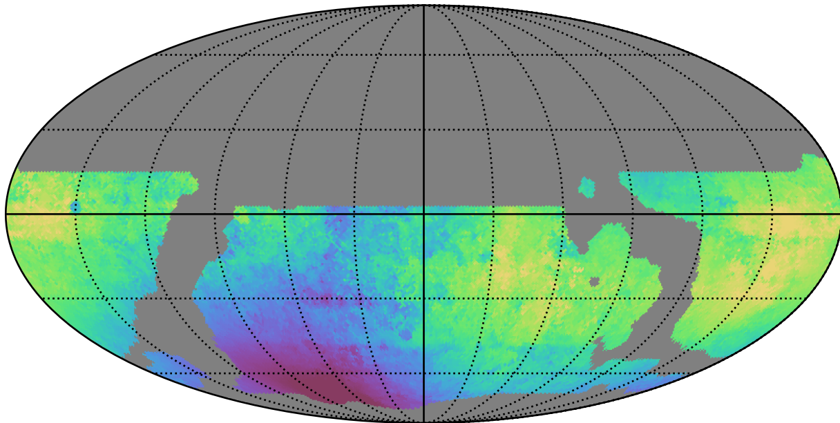
weather_cloudso14v3.4_10yrs WFD g band: Median solarElong
