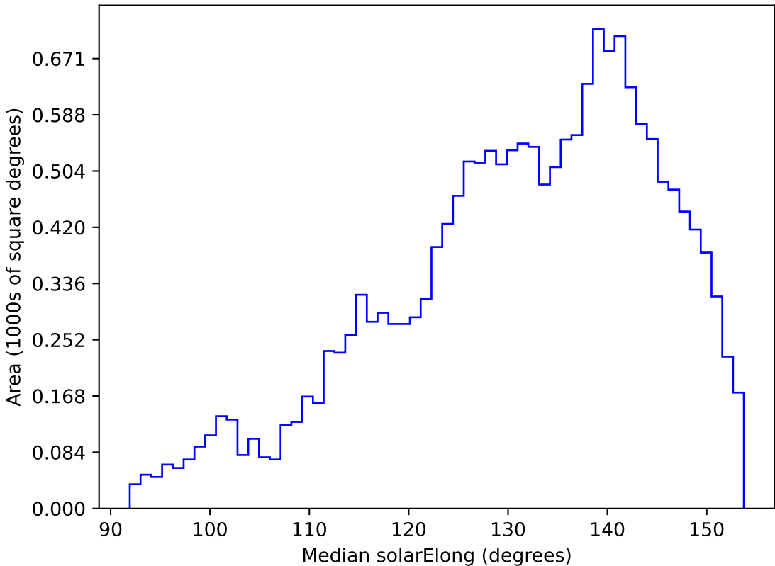
weather_cloudso14v3.4_10yrs WFD g band: Median solarElong
