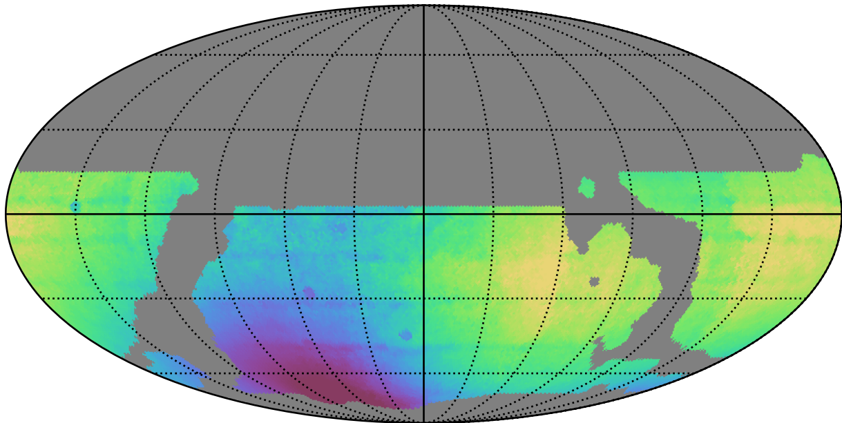
weather_cloudso14v3.4_10yrs WFD all bands: Median solarElong
