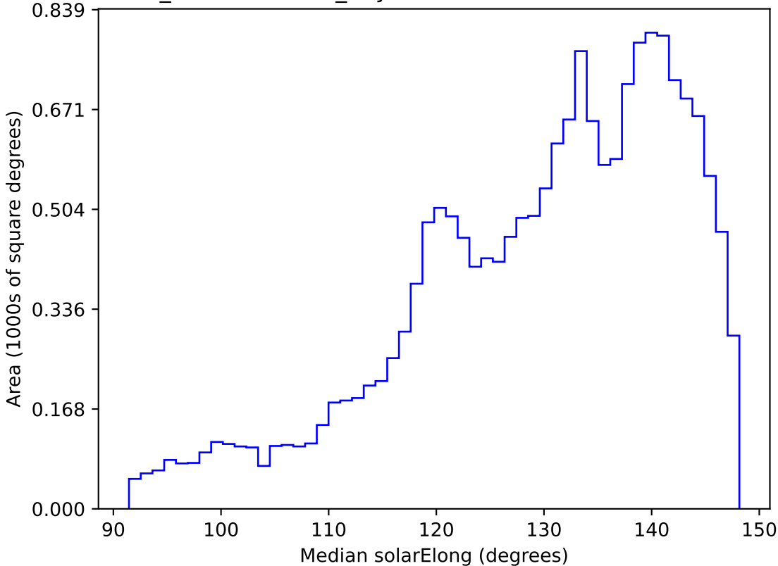
weather_cloudso14v3.4_10yrs WFD all bands: Median solarElong
