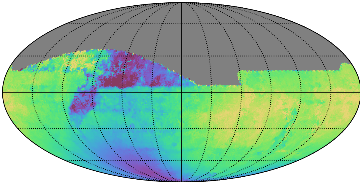
weather_cloudso14v3.4_10yrs All sky z band: Median solarElong
