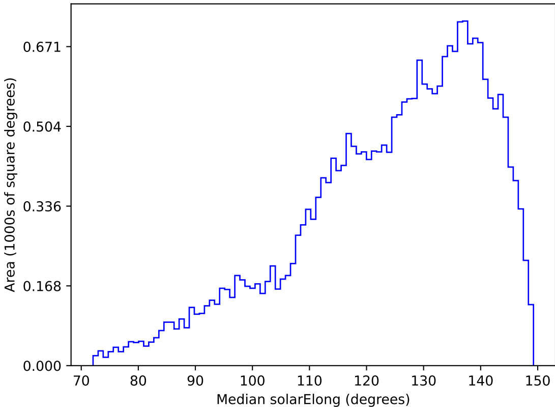
weather_cloudso14v3.4_10yrs All sky z band: Median solarElong
