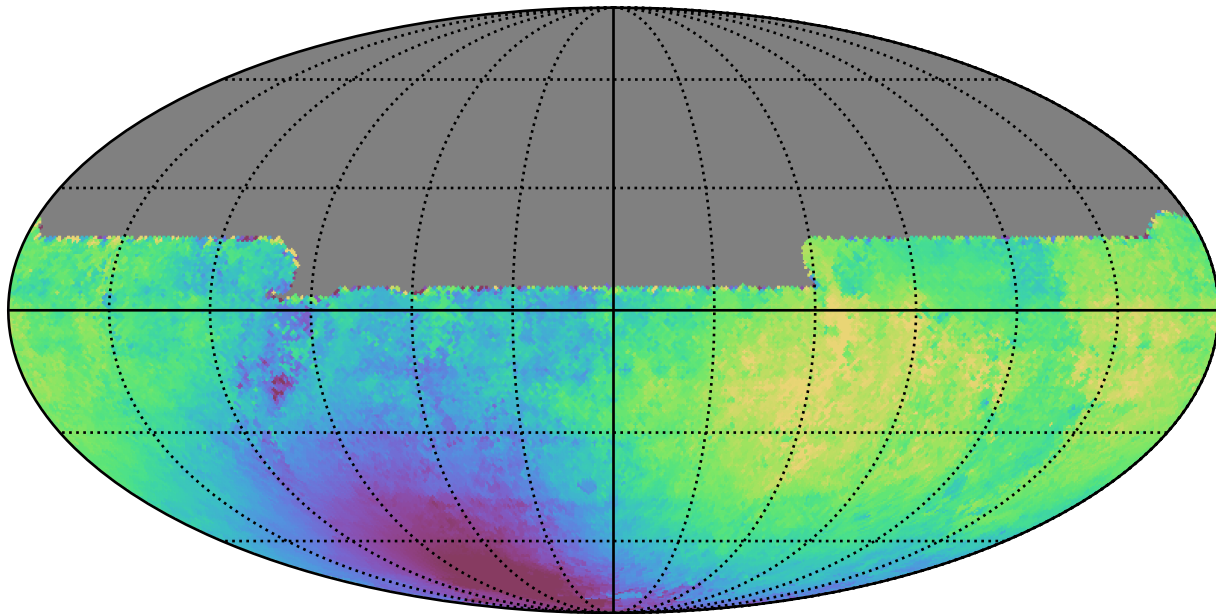
weather_cloudso14v3.4_10yrs All sky y band: Median solarElong
