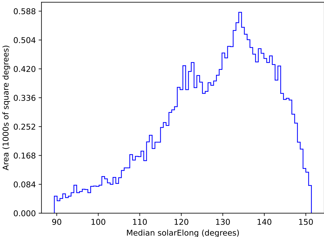
weather_cloudso14v3.4_10yrs All sky y band: Median solarElong
