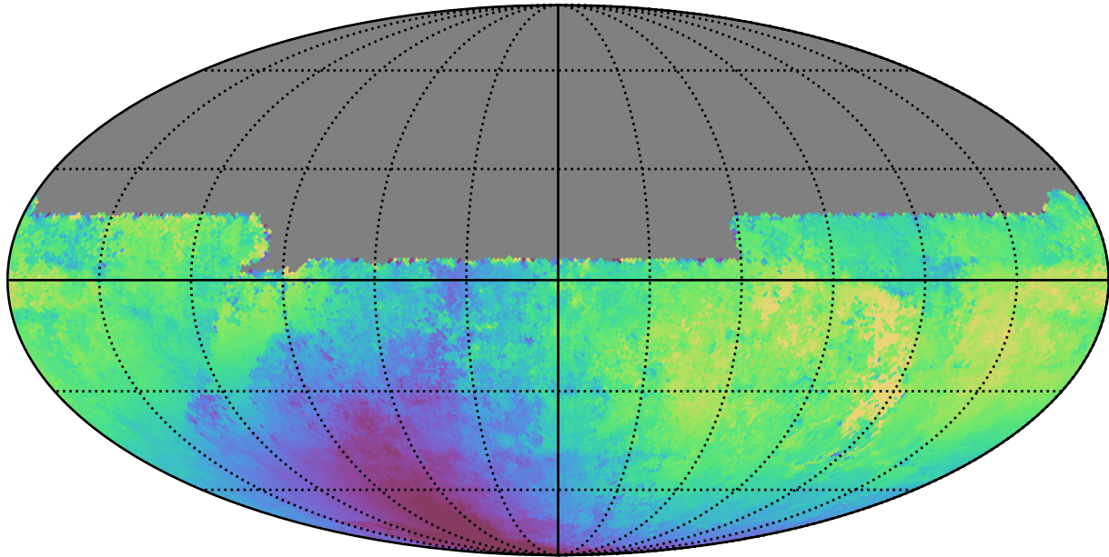
weather_cloudso14v3.4_10yrs All sky u band: Median solarElong
