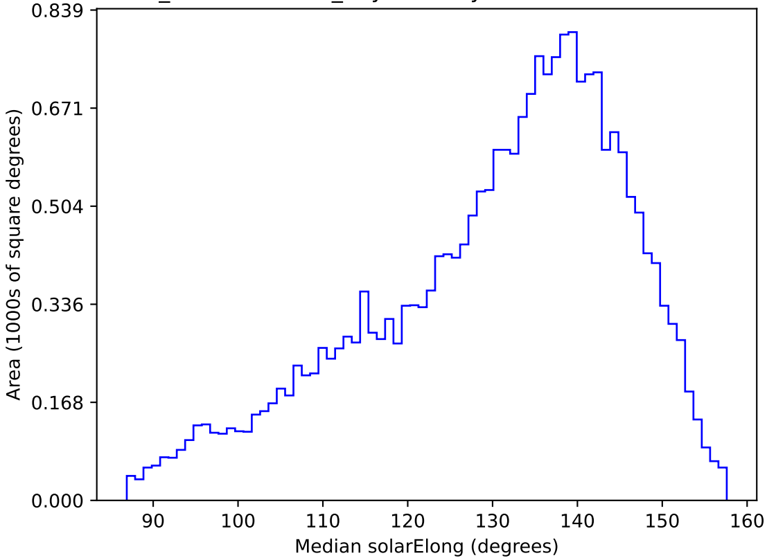
weather_cloudso14v3.4_10yrs All sky u band: Median solarElong
