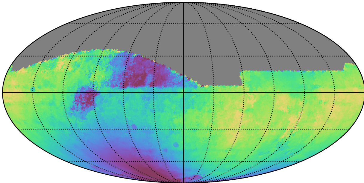
weather_cloudso14v3.4_10yrs All sky r band: Median solarElong
