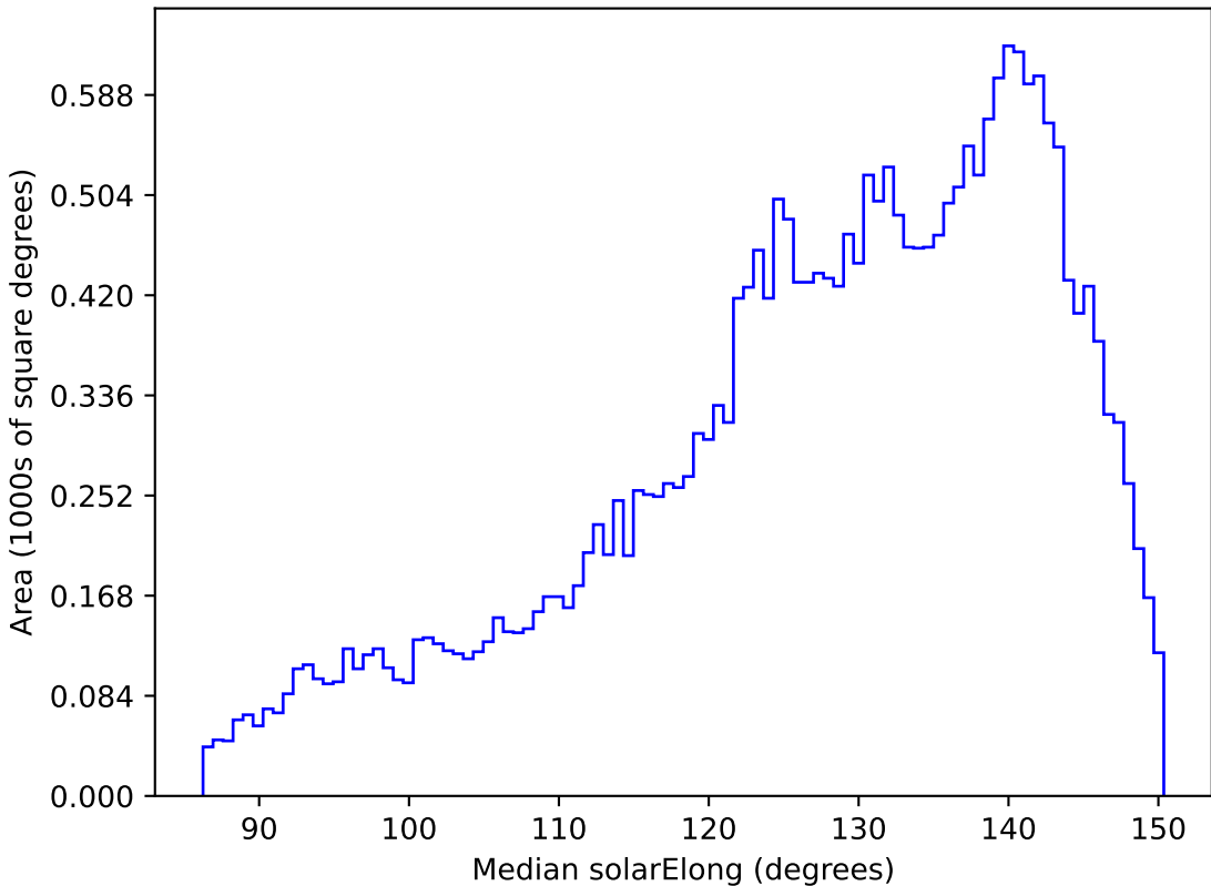
weather_cloudso14v3.4_10yrs All sky r band: Median solarElong
