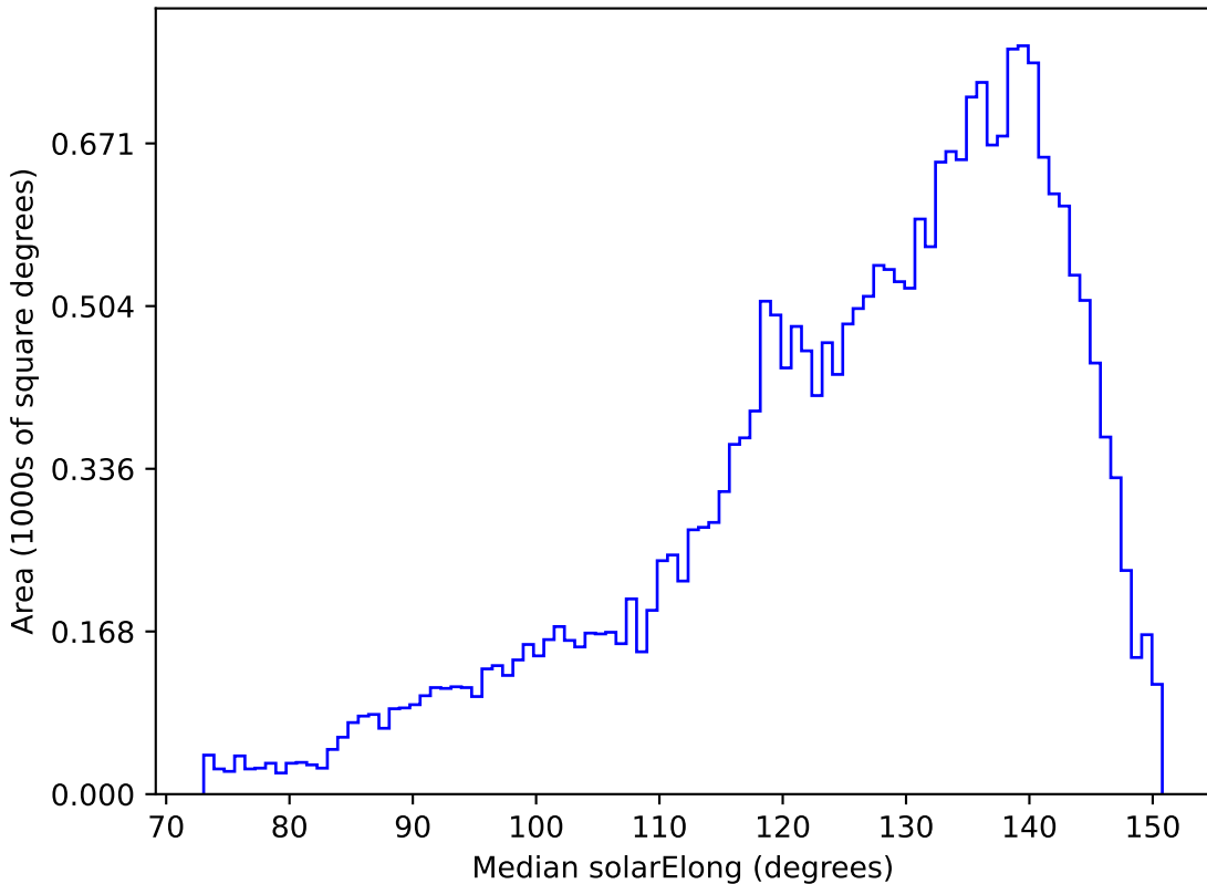
weather_cloudso14v3.4_10yrs All sky i band: Median solarElong
