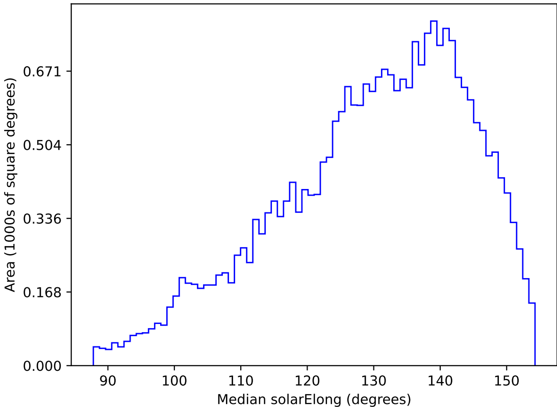
weather_cloudso14v3.4_10yrs All sky g band: Median solarElong
