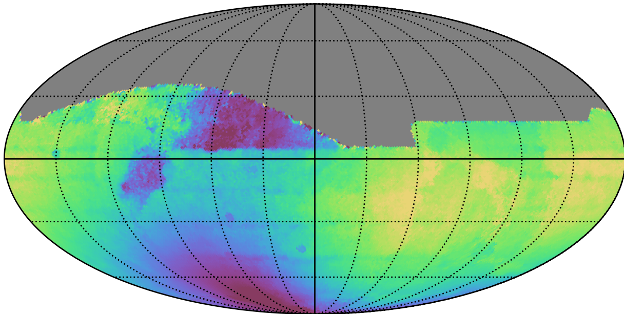
weather_cloudso14v3.4_10yrs All sky all bands: Median solarElong
