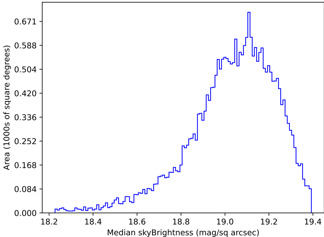
weather_cloudso14v3.4_10yrs Yr 1 z band: Median skyBrightness
