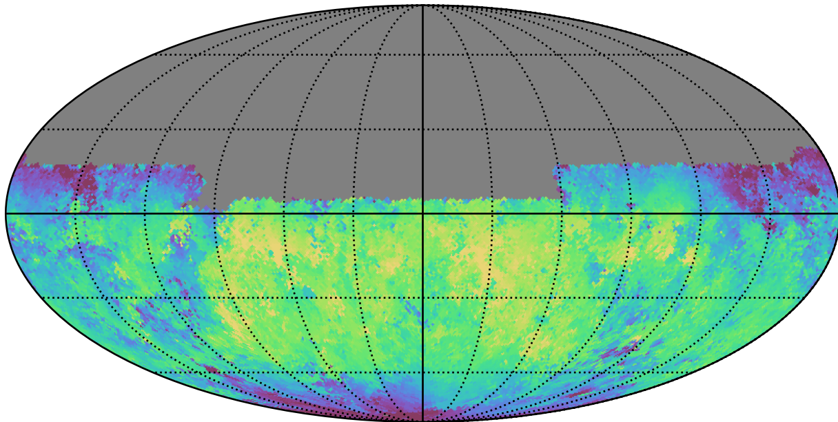
weather_cloudso14v3.4_10yrs Yr 1 y band: Median skyBrightness
