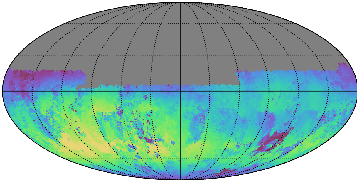
weather_cloudso14v3.4_10yrs Yr 1 u band: Median skyBrightness
