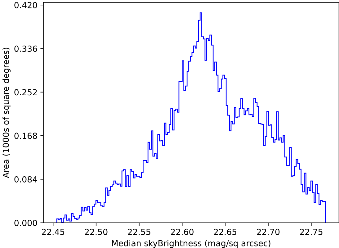
weather_cloudso14v3.4_10yrs Yr 1 u band: Median skyBrightness
