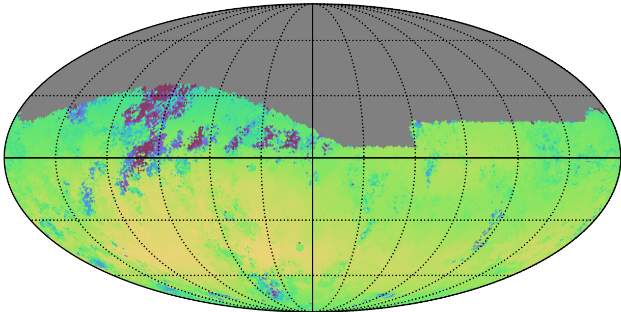
weather_cloudso14v3.4_10yrs Yr 1 r band: Median skyBrightness
