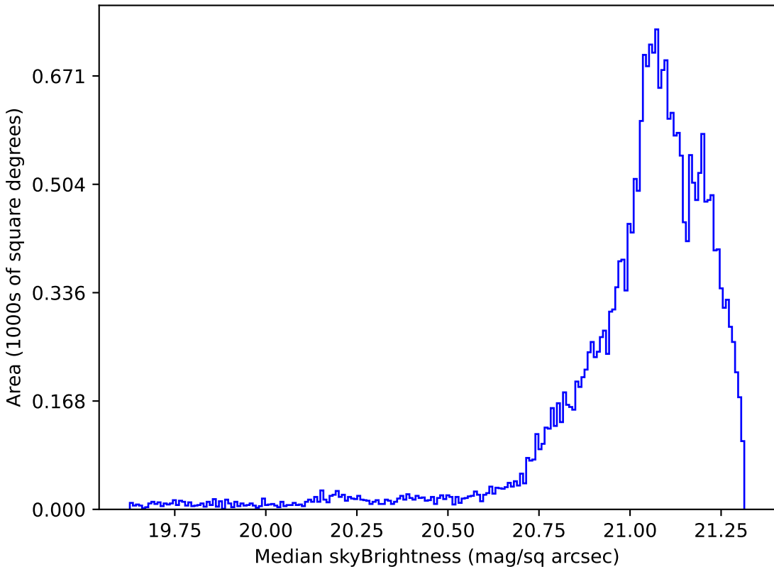
weather_cloudso14v3.4_10yrs Yr 1 r band: Median skyBrightness
