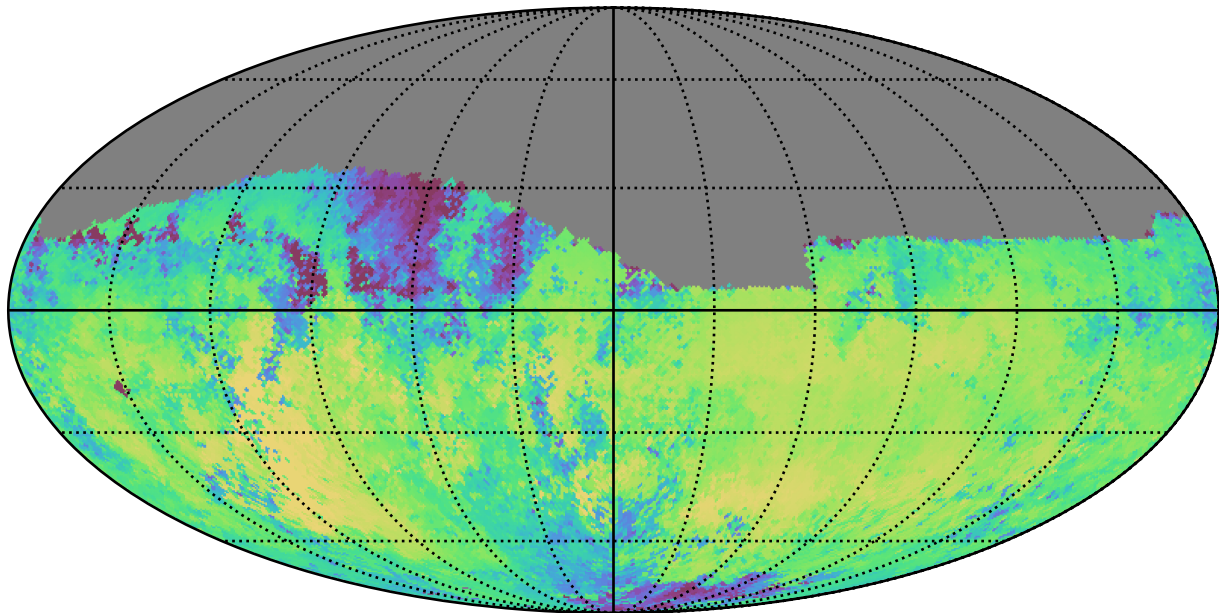
weather_cloudso14v3.4_10yrs Yr 1 i band: Median skyBrightness
