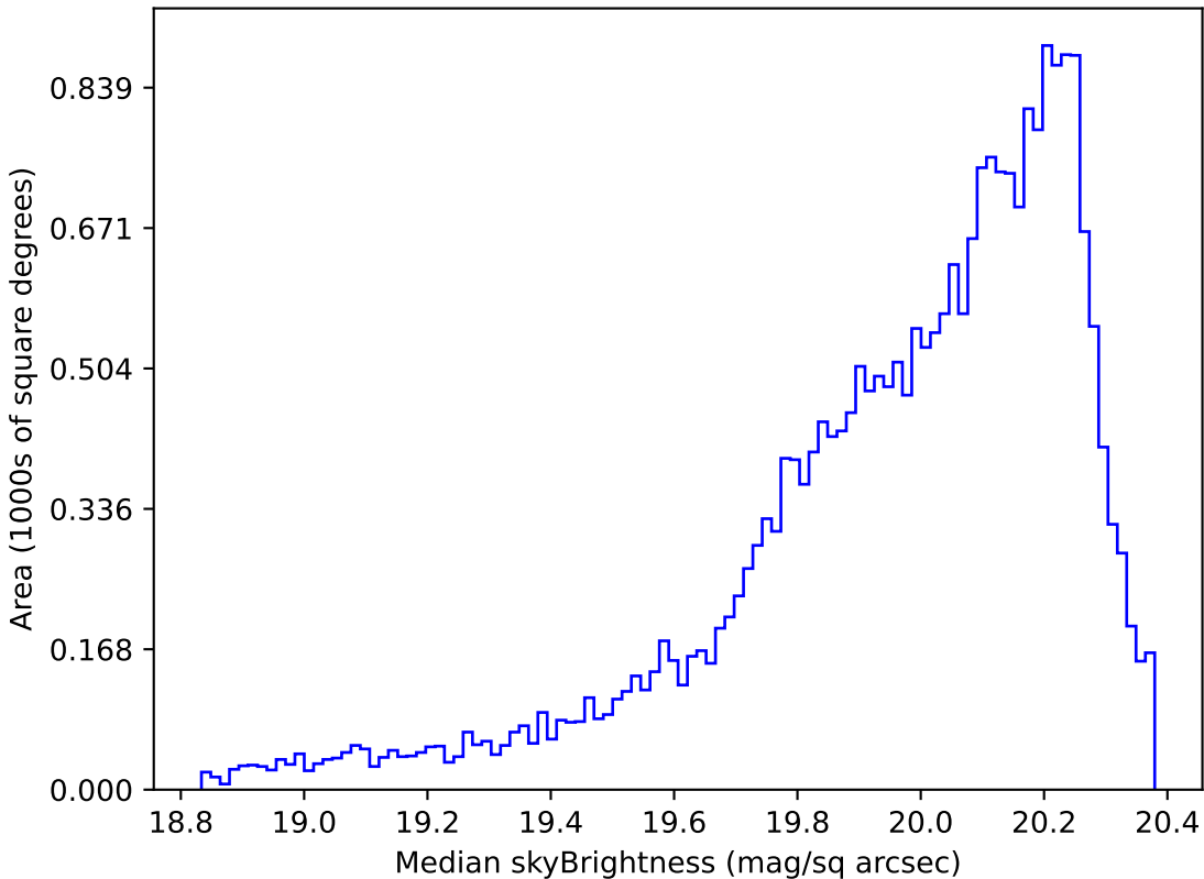
weather_cloudso14v3.4_10yrs Yr 1 i band: Median skyBrightness
